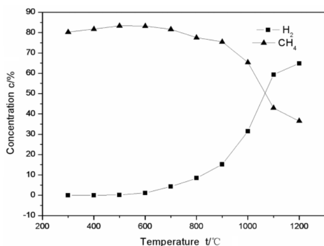
Fig. 4. The concentration of \text{H}_2 , \text{CH}_4 and Pyrolysis temperature in natural gas atmosphere (the concentration of \text{CH}_4 included the effect of atmosphere).
